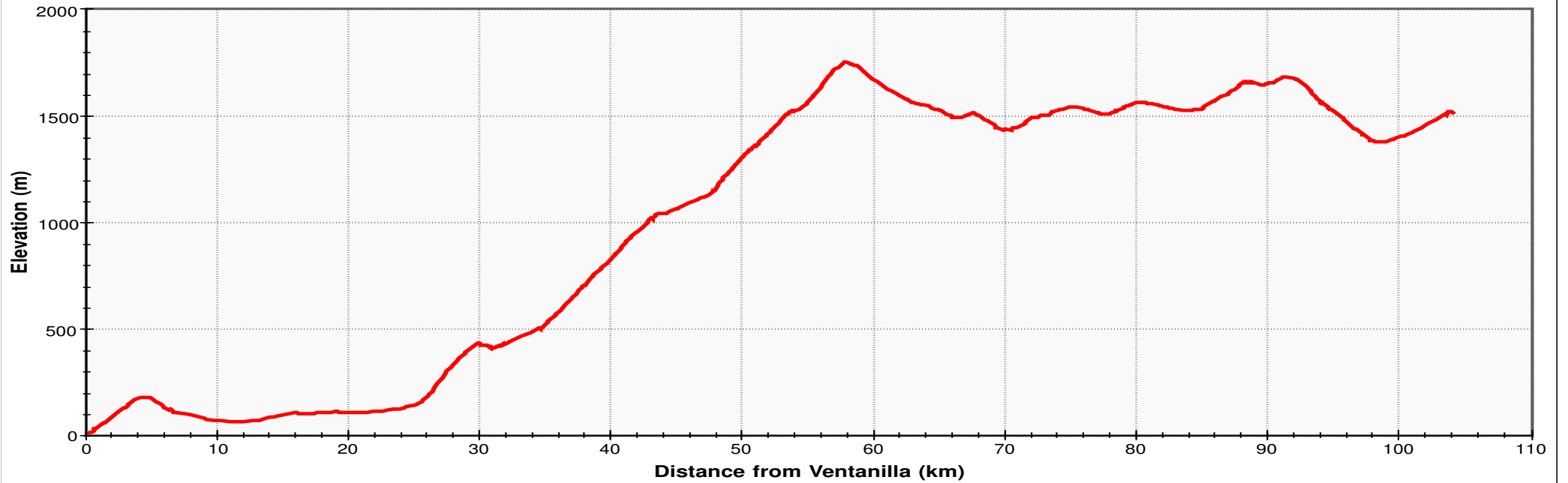
Autopista Elevations
